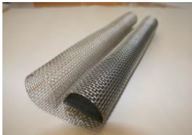
Fig.1 FB Cavity Vents with a single intumescent Sealmaster strip.
